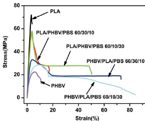
Figure 1. Tensile stress–strain curves of neat PLA, PHBV, and PLA/PHBV/PBS ternary blends.
